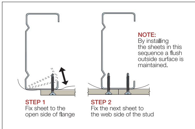
FIGURE 7 SCREW FASTENING
