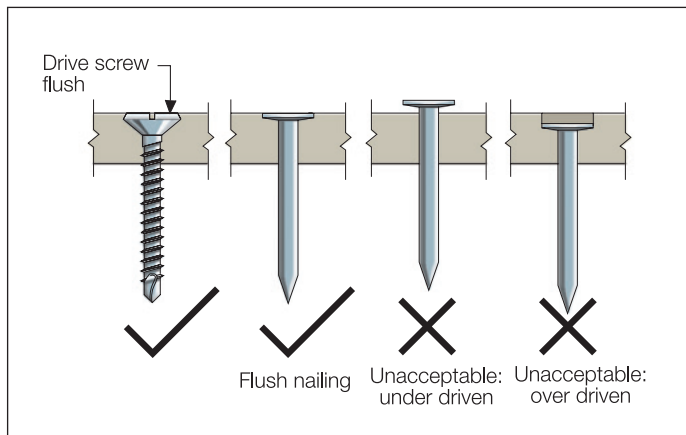
FIGURE 6 FASTENER DEPTH
