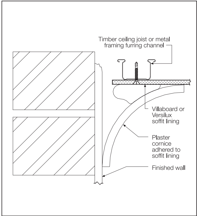
FIGURE 30 CEILING CORNICE
