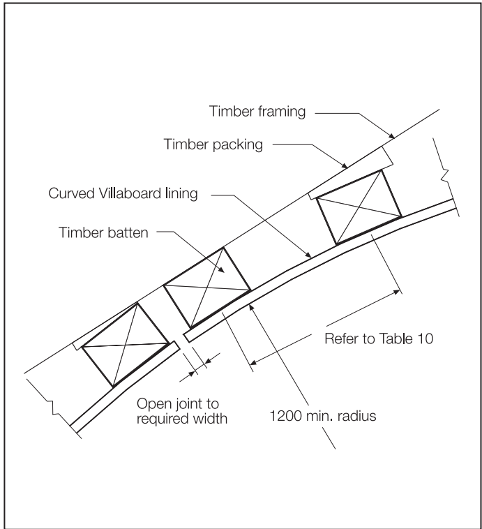
FIGURE 31 CURVED SOFFIT
