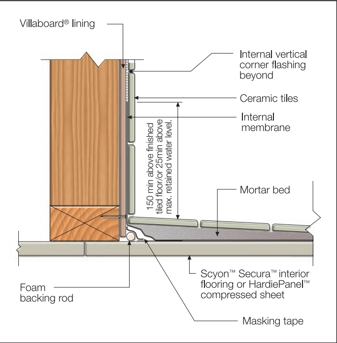
FIGURE 14 IN-SITU APPLIED INTERNAL MEMBRANE
