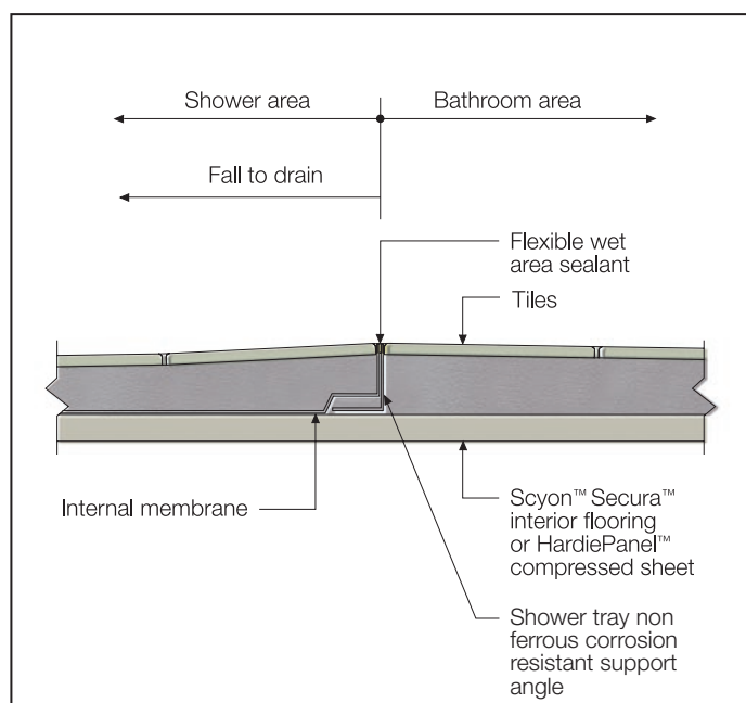
FIGURE 22 UNENCLOSED SHOWER - EDGE FINISHING DETAIL
