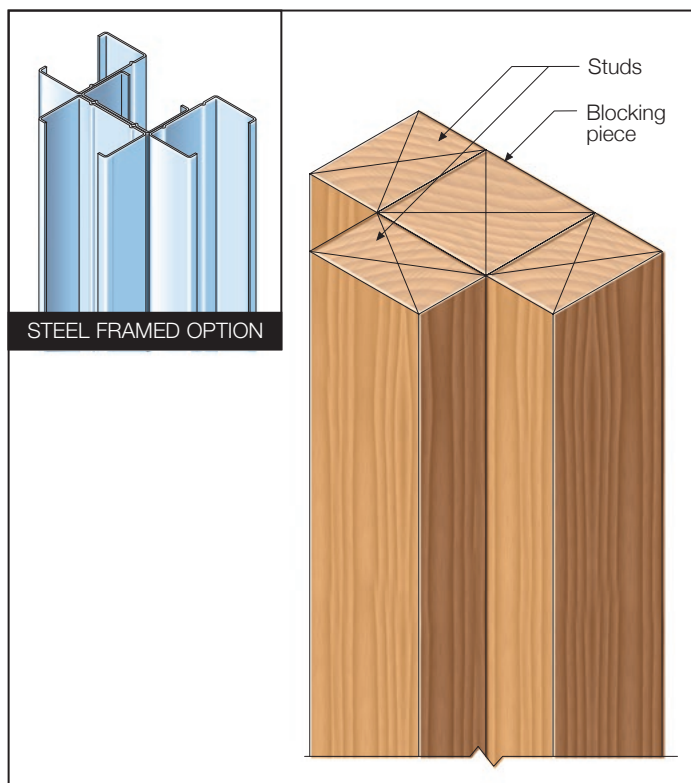
FIGURE 2 BLOCKED CORNER
