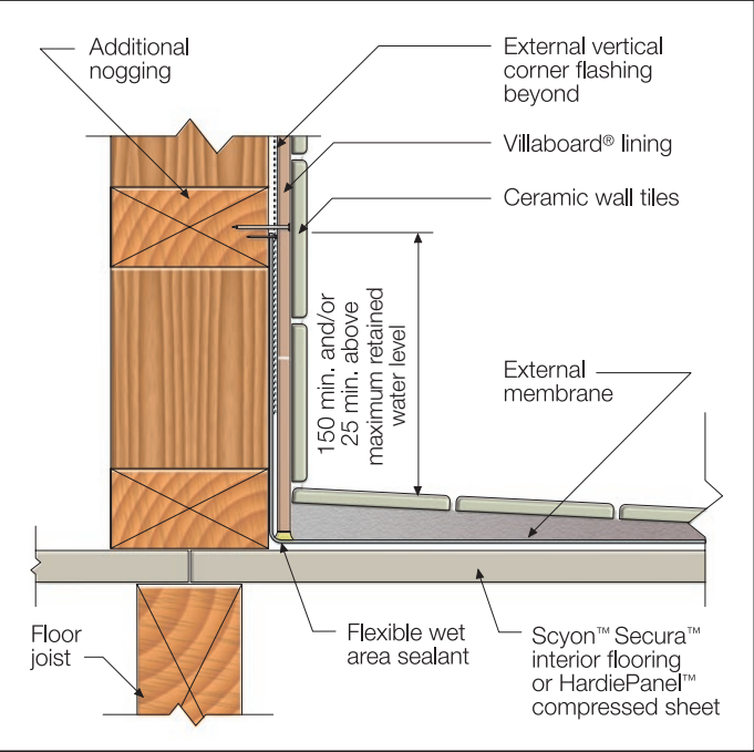
FIGURE 12 EXTERNAL MEMBRANE - VILLABOARD LINING
