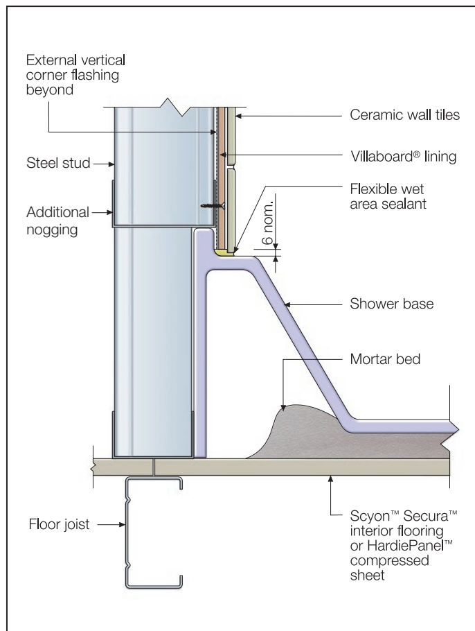
FIGURE 13B PREFORMED TRAY DETAIL FOR VILLABOARD LINING TO BE TILED - STEEL FRAME
