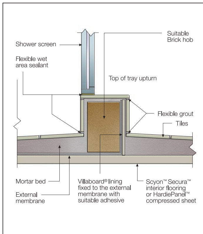
FIGURE 18 BRICK HOB - EXTERNAL MEMBRANE
