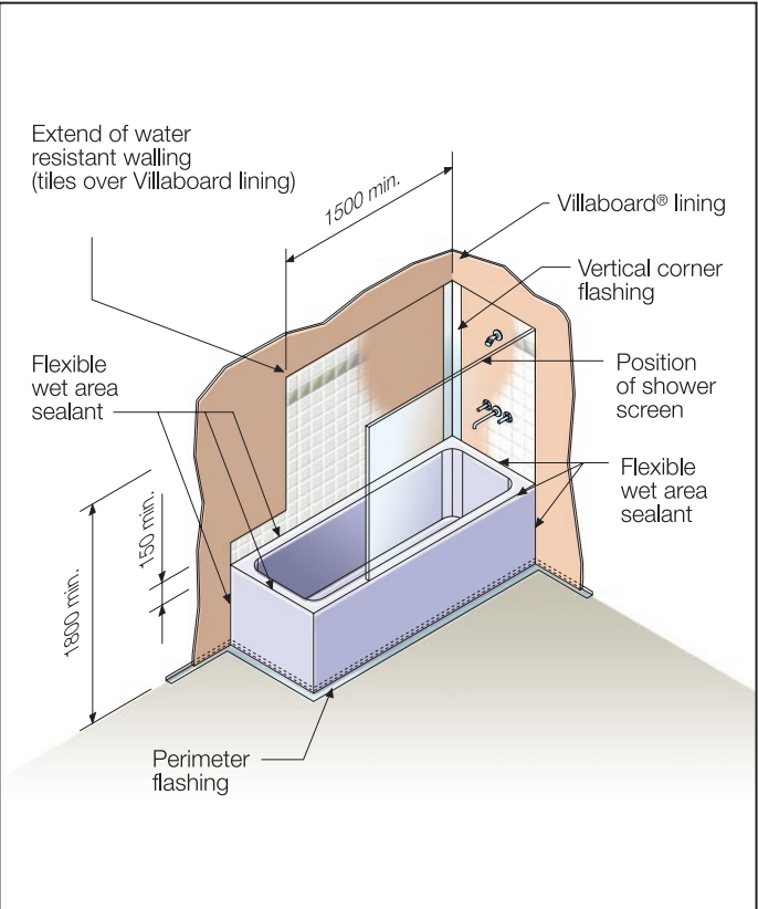
FIGURE 16 SHOWER OVER BATH - WITH SHOWER SCREEN
