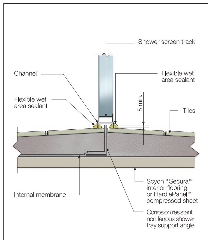
FIGURE 19 HOBLESS SHOWER
