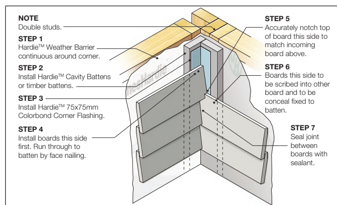
FIGURE 13 INTERNAL CORNER NOTCH & SCRIBE OPTION
