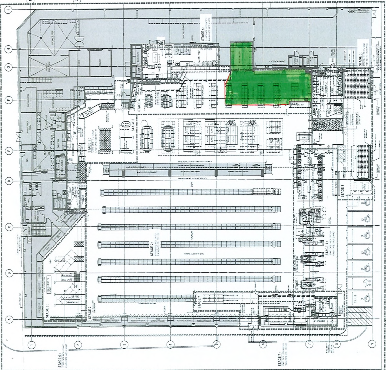
1 GROUND FLOOR PLAN - OVERLAY EXISTING & PROPOSED
