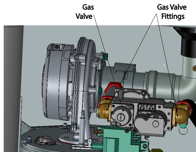
Fig. 4: Instinct 110 Floor Standing Boiler
