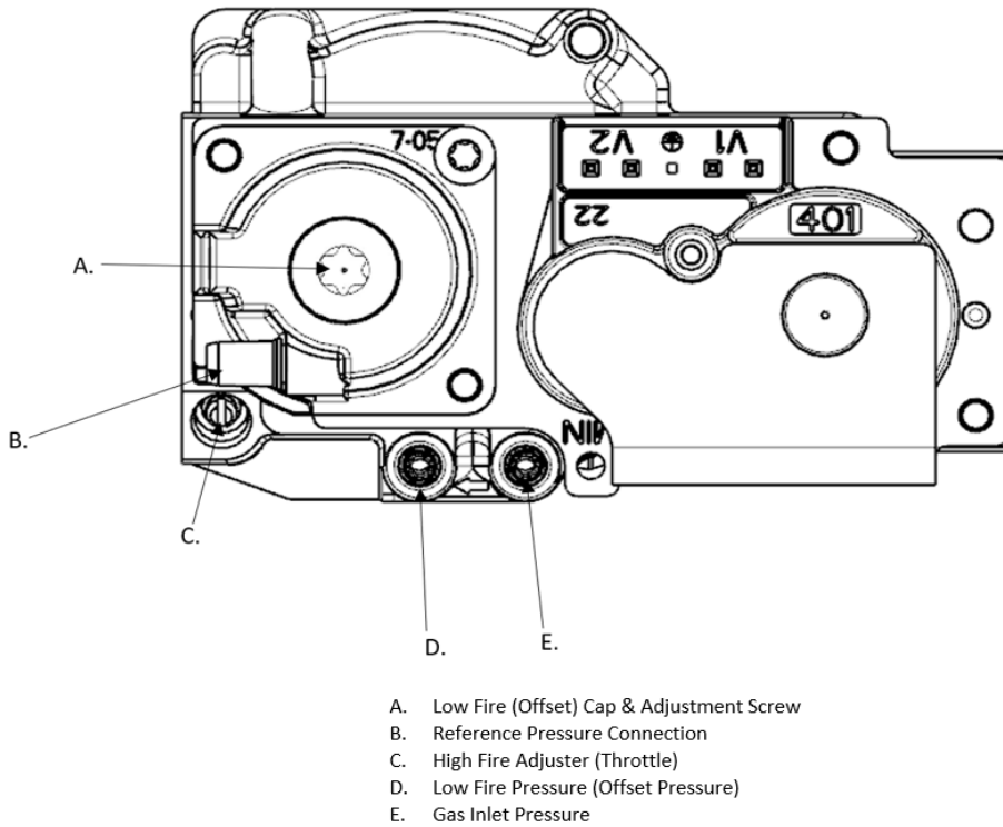
Fig. 10: Throttle Screw Location
