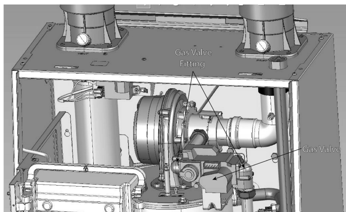
Fig. 1: Instinct 110 Wall Hung Boiler
