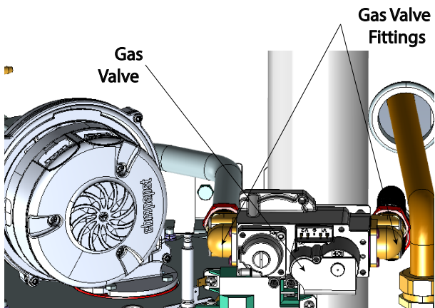
Fig. 5: Instinct 155 Floor Standing Boiler
