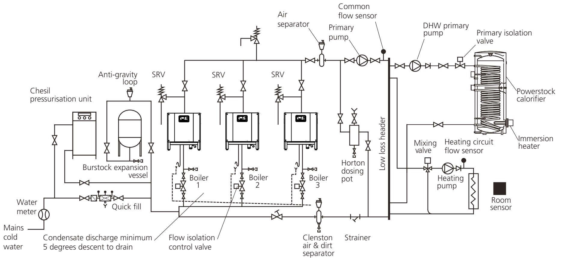
Scheme 4: Sealed system with flow isolation valves and a low loss header.
