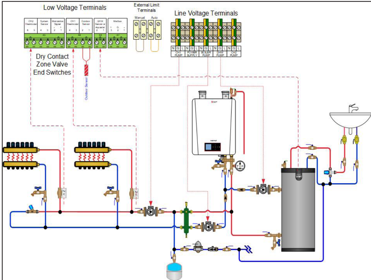
Fig. 23: Instinct Solo - Piping with Zone Valves - Domestic Piping Alternate
