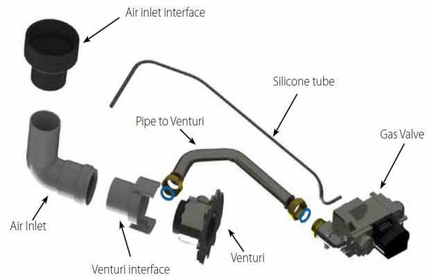
Fig. 2: Instinct 155 Gas Train
