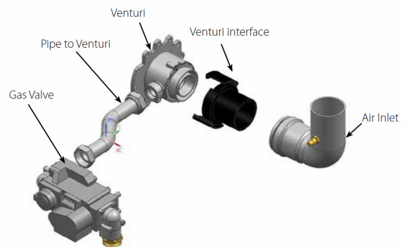
Fig. 3: Instinct 199 Gas Train
