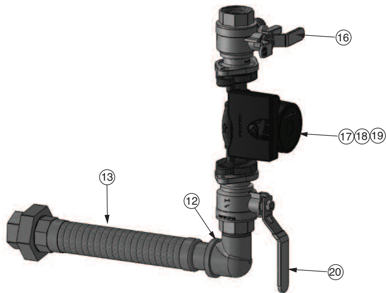
Fig. 12: Cascade Kit Components for Solo 399 Boilers – Primary Secondary Return Piping - See Table 4, Page 13
