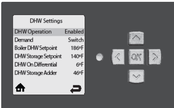
Fig. 7: DHW Settings
