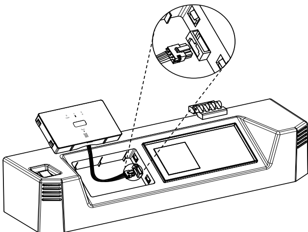
Fig. 13: 8-way harness
