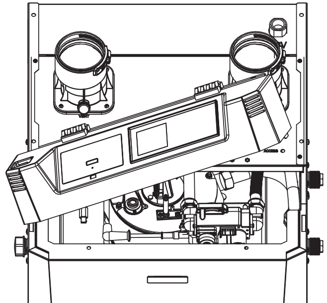
Fig. 11: HMI Removal
