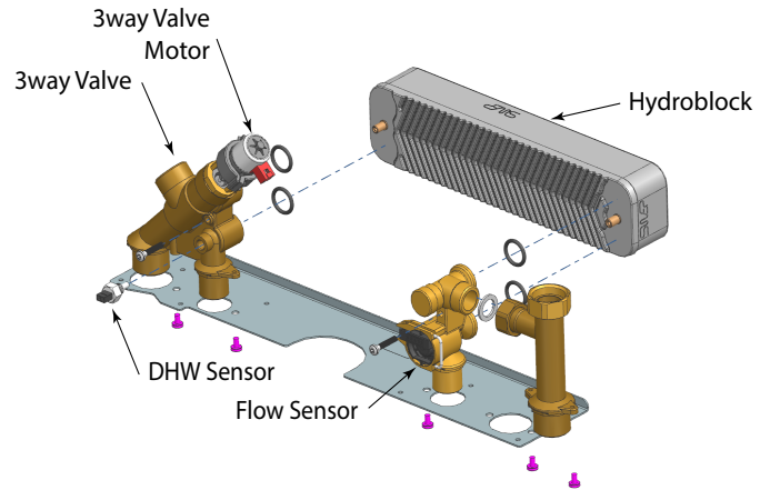
Fig. 2: Hydroblock Assembly
