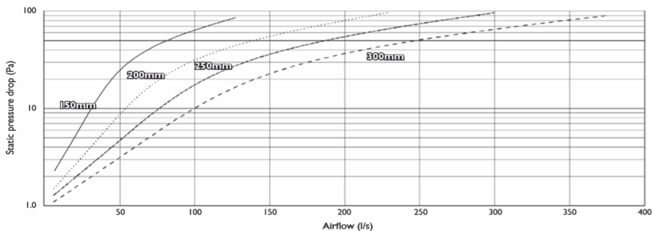
Static pressure drop versus airflow
