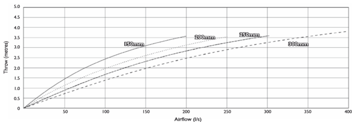
Throw versus airflow
