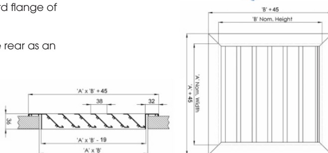
MODEL OAL-S - Stock Sizes Available
