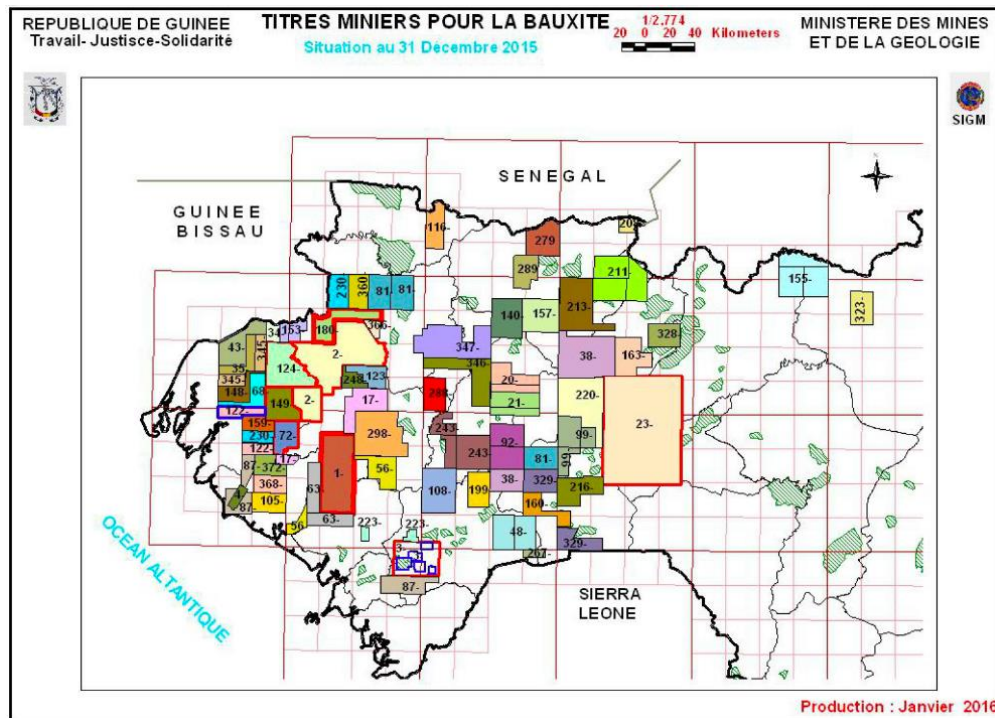
Figure 3. Bauxite mining map of Guinea ( https://mines.gov.gn/en/media/maps/ ). The Global Alumina Corporation concessions is #124 and the CBG concession is #2
