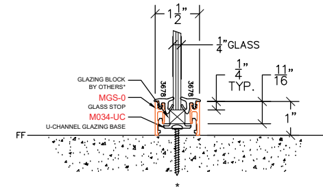
M420 - GLAZING SILL
