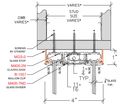
M400 - GLAZING HEAD
