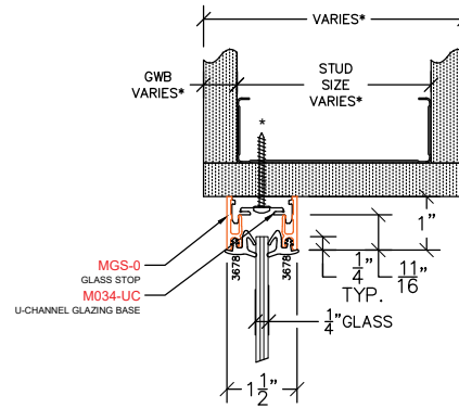
M400 - GLAZING JAMB
