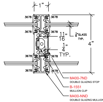
M305 - GLAZING VERTICAL
