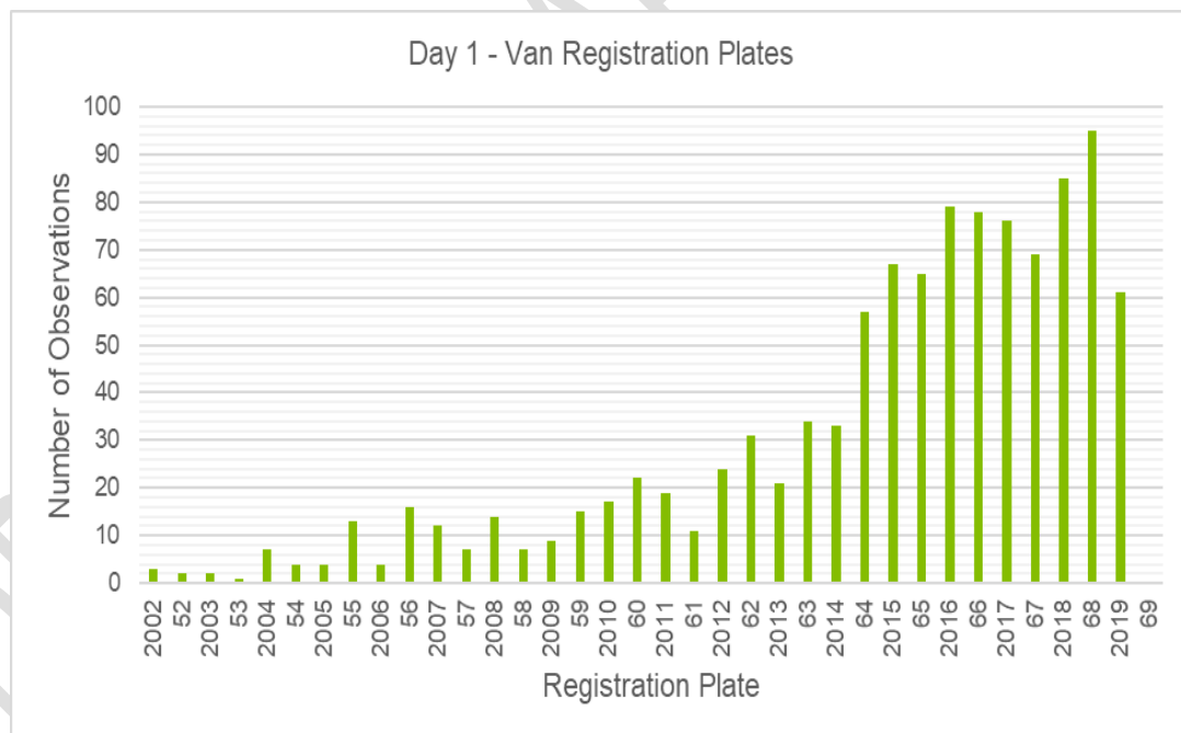
Figure 2-4 Bridge Street/Deansgate van registration years
