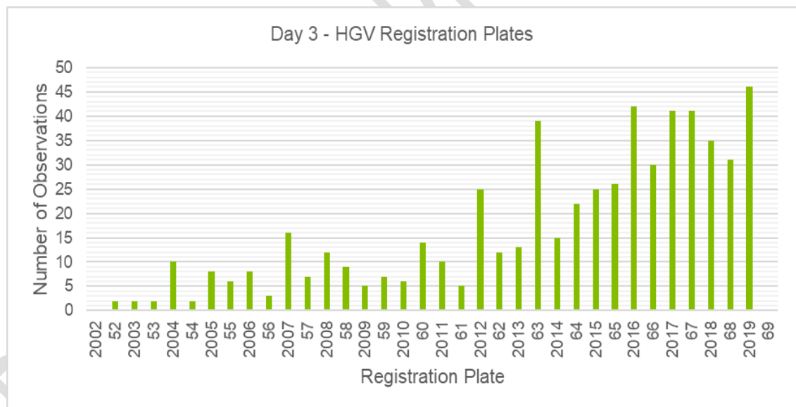
Figure 4-5 A6/Grosvenor Street HGV registration years
