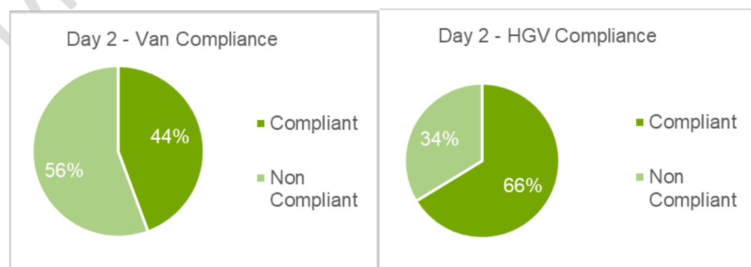
Figure 3-3 Regent Road/Ordsall Lane vehicle compliance splits
