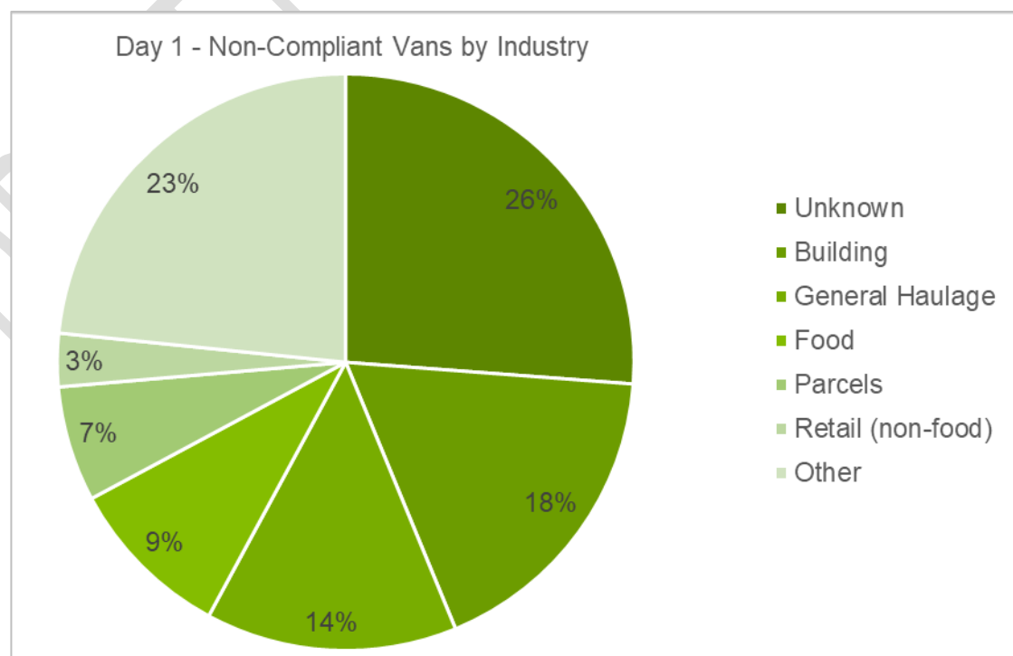
Figure 2-6 Bridge Street/Deansgate non-compliant vans by industry
