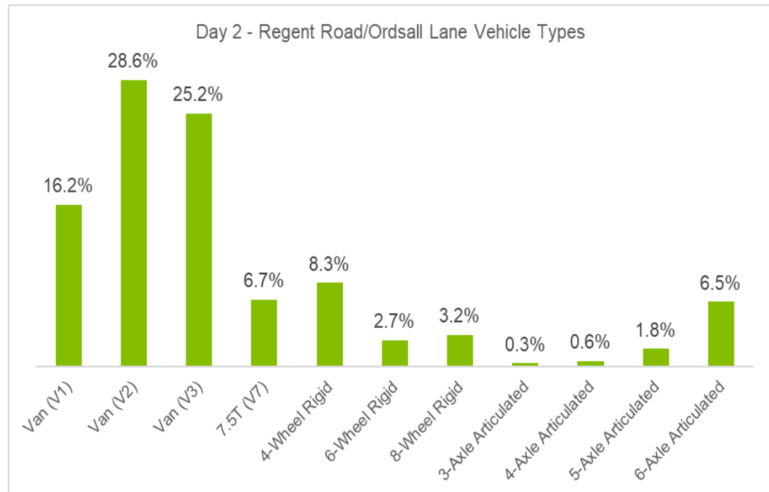
Figure 3-2 Regent Road/Ordsall Lane Vehicle Type Splits
