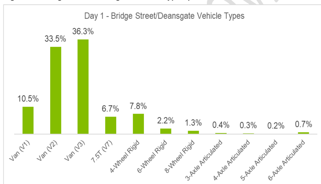
Figure 2-2 Bridge Street/Deansgate Vehicle Type Split
