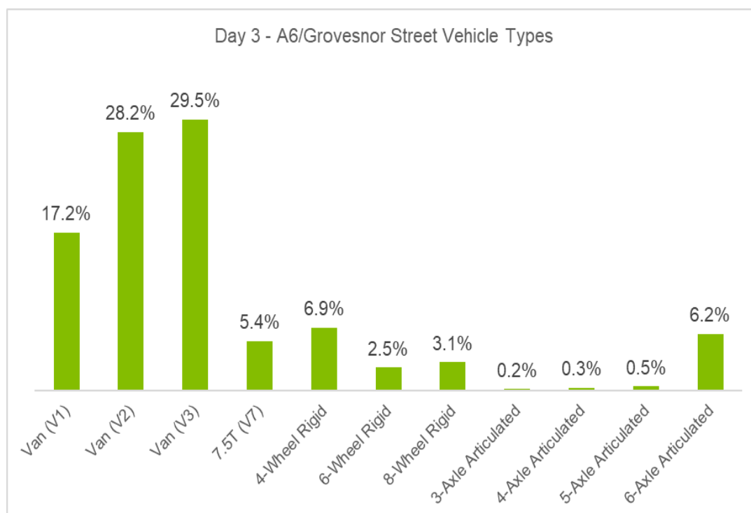
Figure 4-2 A6/Grosvenor Street Vehicle Type Split
