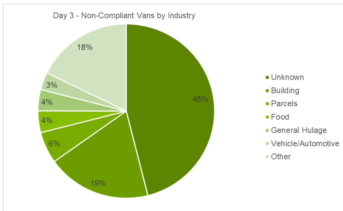
Figure 4-6 A6/Grosvenor Street non-compliant vans by industry
