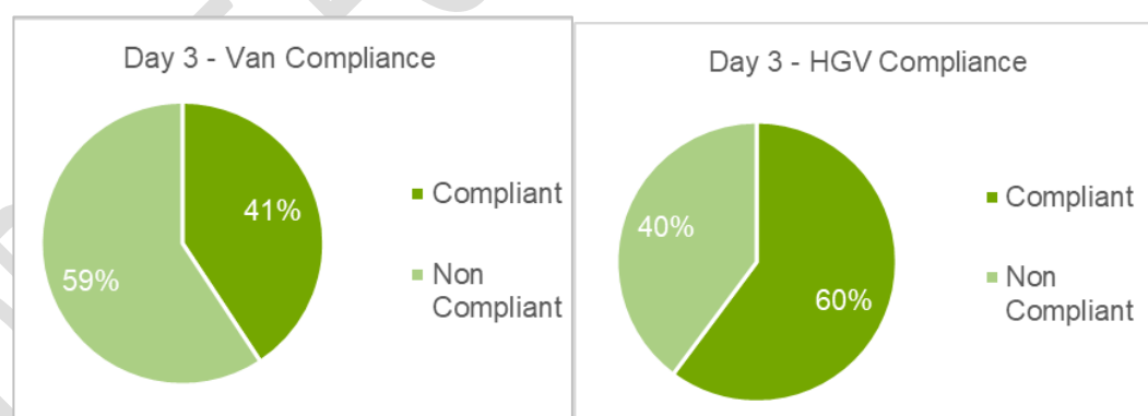
Figure 4-3 A6/Grosvenor Street vehicle compliance splits
