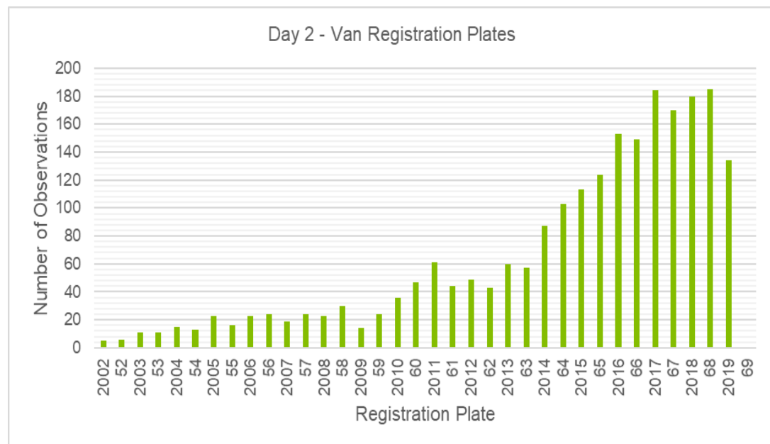
Figure 3-4 Regent Road/Ordsall Lane van registration years
