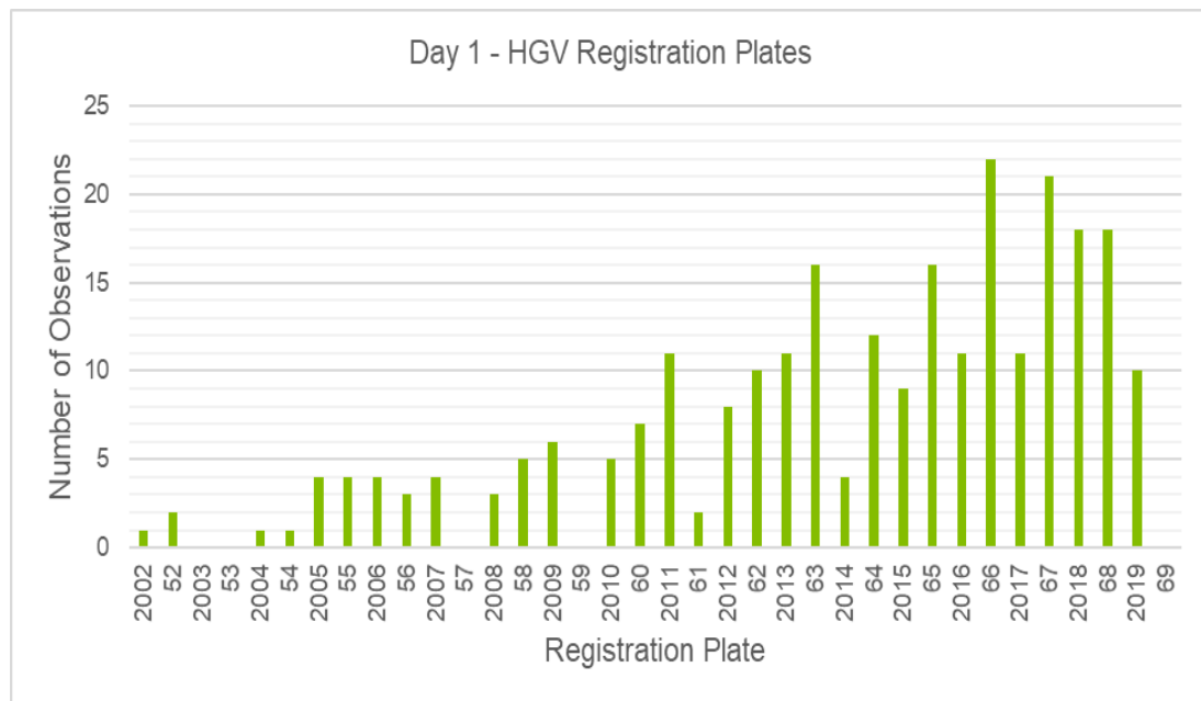
Figure 2-5 Bridge Street/Deansgate HGV registration years
