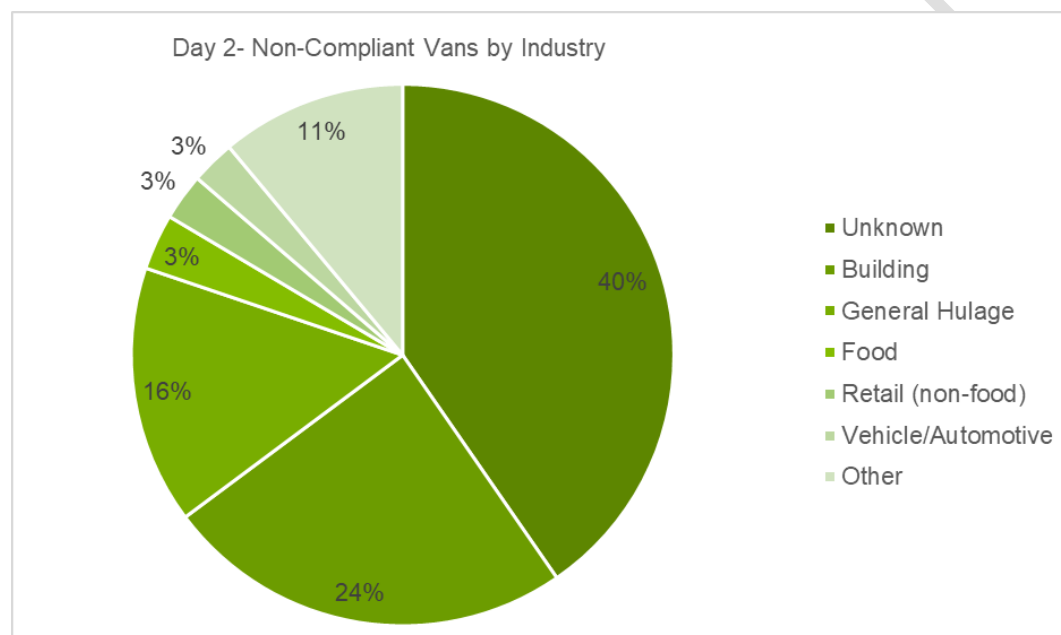
Figure 3-6 Regent Road/Ordsall Lane non-complaint vehicles by industry
