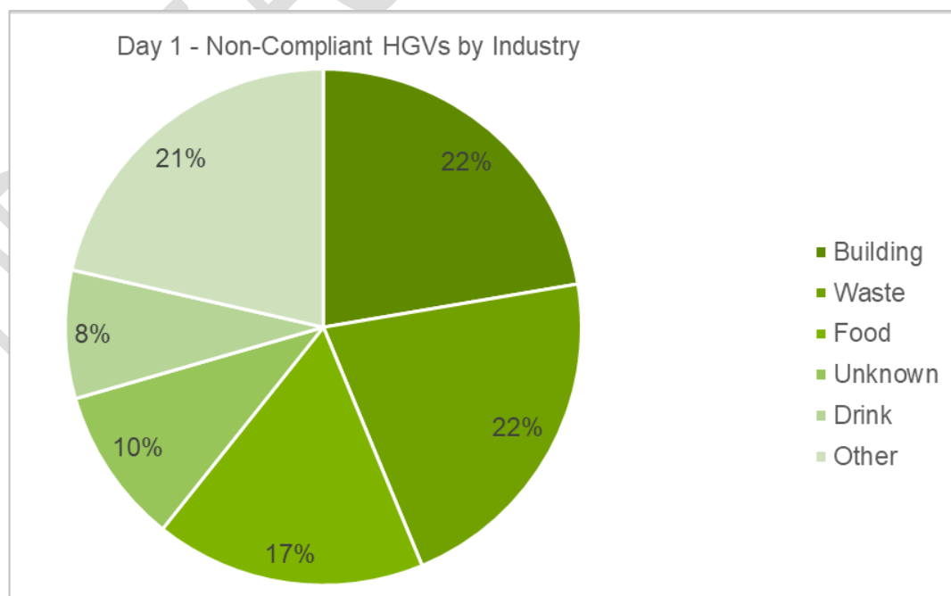
Figure 2-7 Bridge Street/Deansgate non-compliant HGVs by industry
