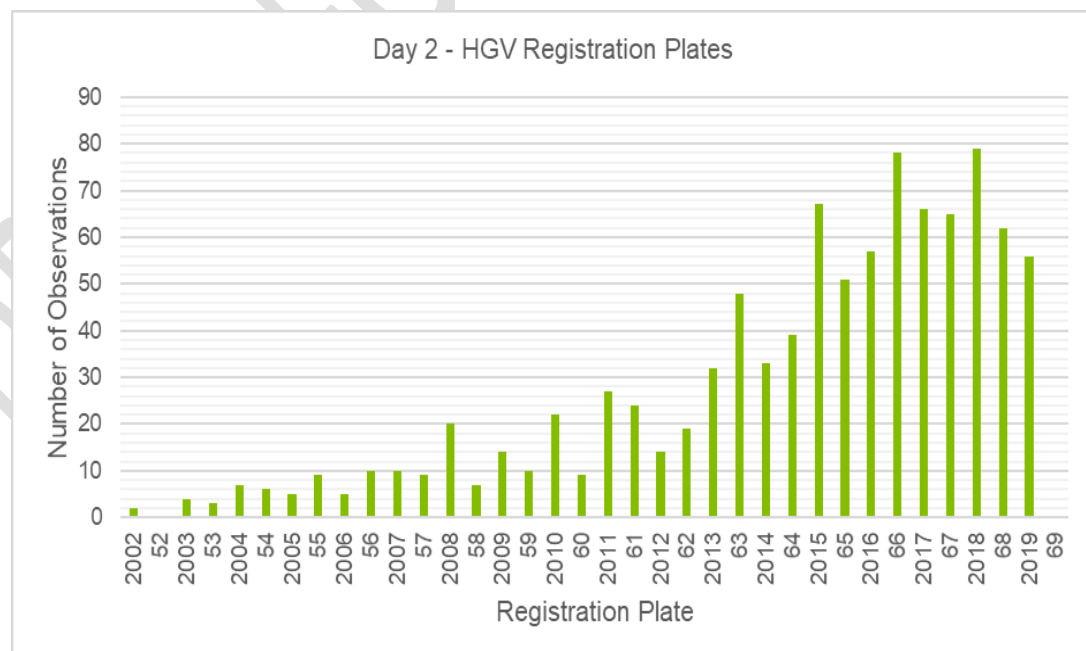
Figure 3-5 Regent Road/Ordsall Lane HGV registration years
