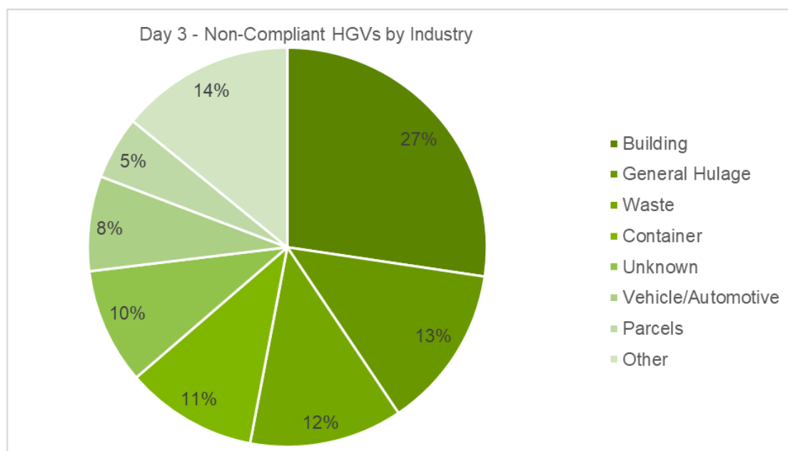
Figure 4-7 A6/Grosvenor Street non-compliant HGVs by industry
