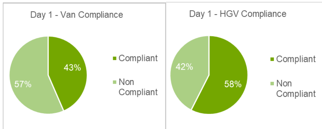
Figure 2-3 Bridge Street/Deansgate van compliance split
