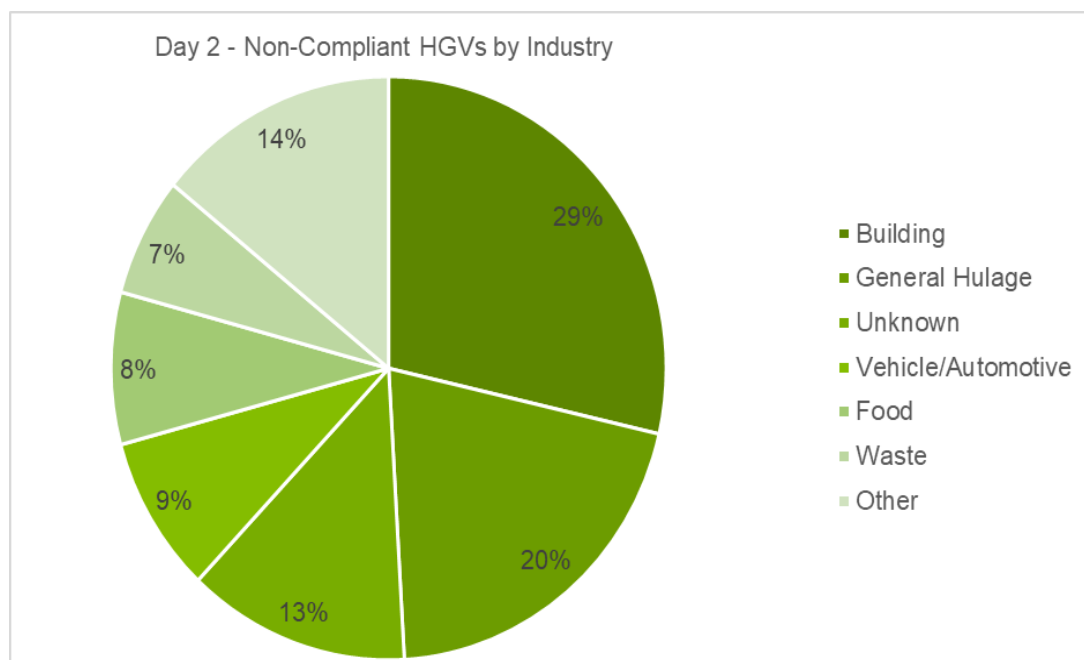
Figure 3-7 Regent Road/Ordsall Lane non-compliant vehicles by industry
