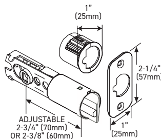
4-IN-1 ENTRY LATCH
