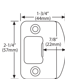
FULL LIP RADIUS STRIKE
