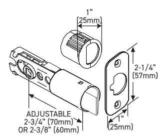
4-IN-1 PRIVACY PASSAGE LATCH
