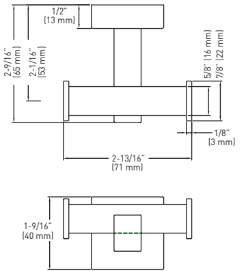
DOUBLE ROBE HOOK
