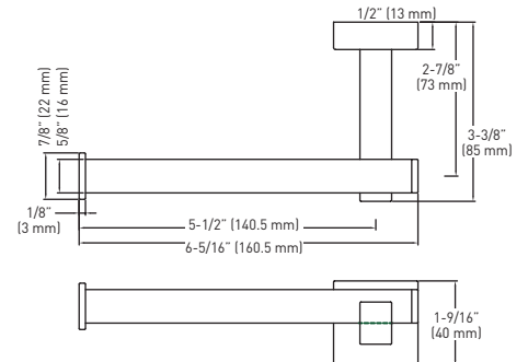
PAPER HOLDER (LEFT HAND INSTALLATION ONLY)
