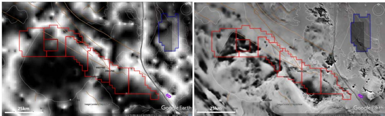
Figure 3. 3a. Gravity (2019 De-Trended Isostatic Residual Gravity 1VD CSCBA (Geoscience Australia)). 3b Magnetics 2019 (TMI Magnetic Grid of Australia 40m cells – Geoscience Australia). Note gravity anomaly in the centre of the gravity image within the Beefwood tenement. (Source: TRP)
