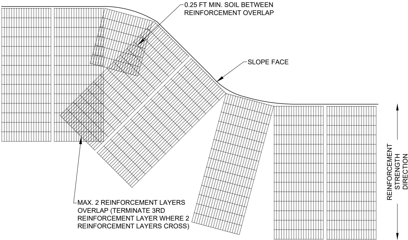
PRIMARY REINFORCEMENT PLACEMENT ON CURVES DETAIL (N.T.S.)
