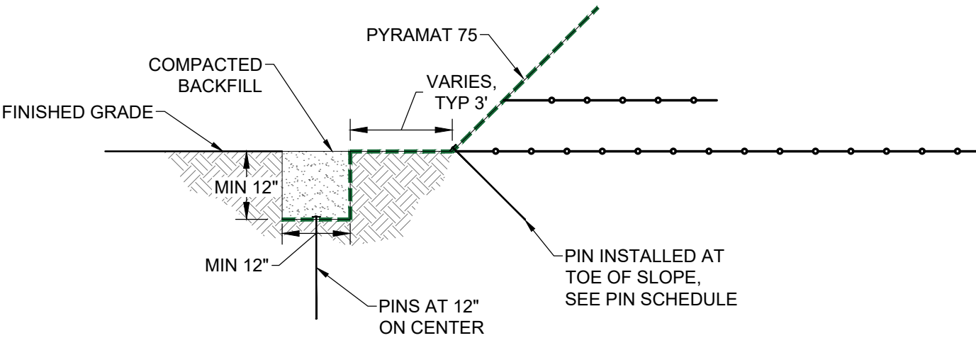
ANCHOR TRENCH AT TOE OF SLOPE
