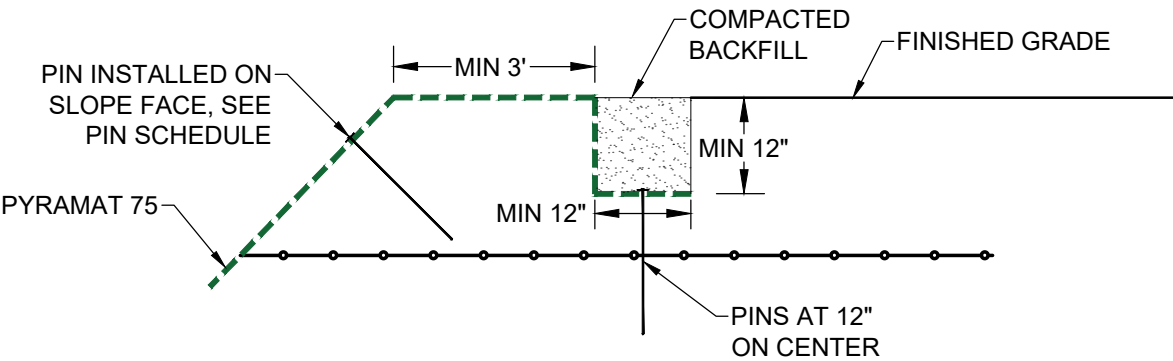
ANCHOR TRENCH AT CREST OF SLOPE
