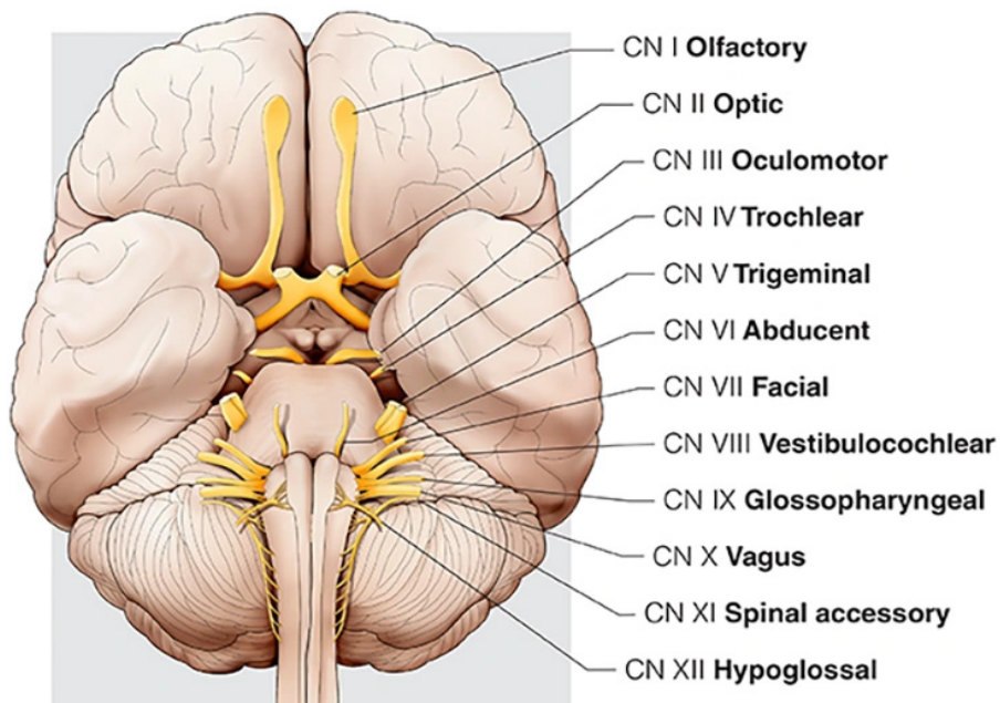
Figure 6 - Cranial Nerves
