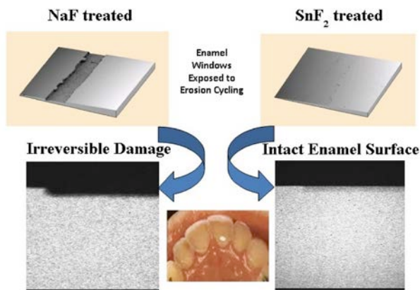
Figure 14. \text{SnF}_2 helps prevent erosion by depositing an acid resistant barrier layer on exposed tooth surfaces, thus preventing the initiation and progression of irreversible damage.
