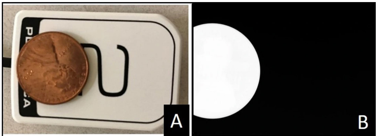
Figure 3 - Digital Sensor (A) Penny placed on active side of sensor. (B) Resultant image shows deadzone with this particular sensor.
