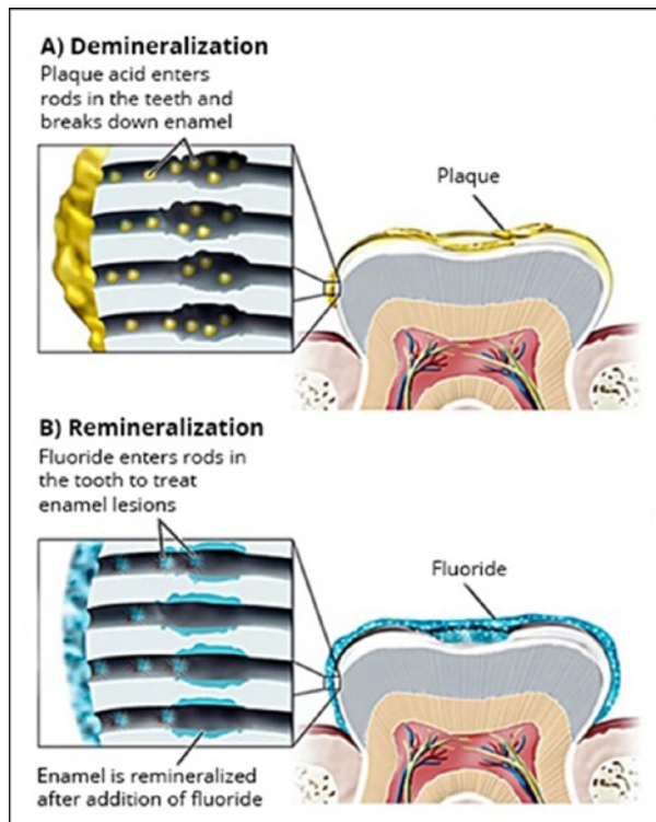
Figure 9. Demineralization/Remineralization. (A) Plaque acids cause a demineralized, sub-surface lesion. (B) Fluoride treatments remineralize the lesion with a more acid resistant fluorapatite mineral.
