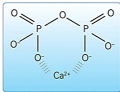
Figure 16. Pyrophosphate. Negatively charged pyrophosphate molecules bind (chelate) positively charged calcium ions.
