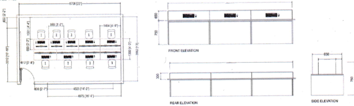
IT ROOM SETUP opt-2 SCALE 1:100
