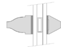
AVAILABLE IN 18MM GLASS SHOWN AS 14MM DOUBLE GLAZED UNIT
