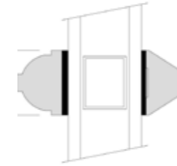
PROFILE AVAILABLE IN 18MM OR 22MM GLASS SHOWN AS 24MM DOUBLE GLAZED UNIT
