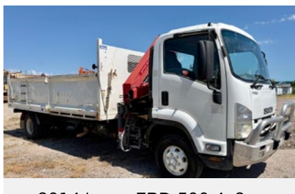
2014 Isuzu FRD 500 4x2 w 2014 HMF 735K3
