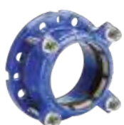
Series 623/10 Supa Plus™ flange adaptor Tensile for PE and uPVC pipes DN40-300 PN10/16 Ductile iron
