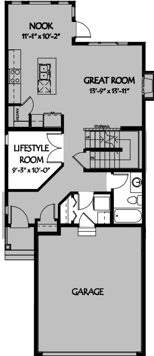
3 3-PIECE BATH & CLOSED-IN LIFESTYLE ROOM
