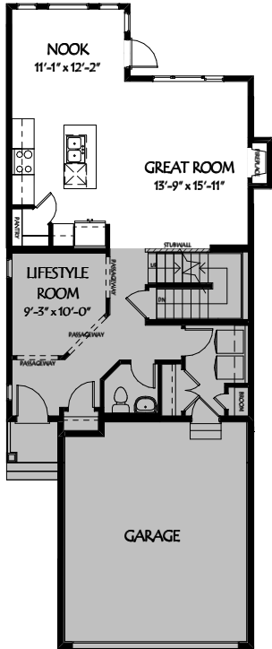
2 2' LENGTH ADDED TO NOOK & GREAT ROOM ADDS 48 SF
