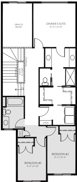
3 OPEN TO BELOW LAYOUT REMOVES 119 SQ. FT
