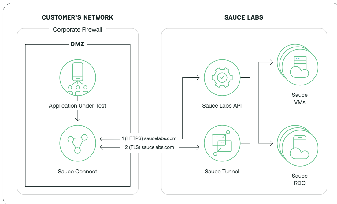
Figure 2: Sauce Connect Proxy, High Level Architecture
