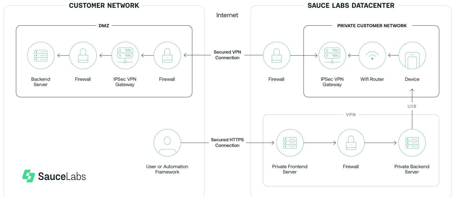
Figure 4: IPSec VPN Data Flow
