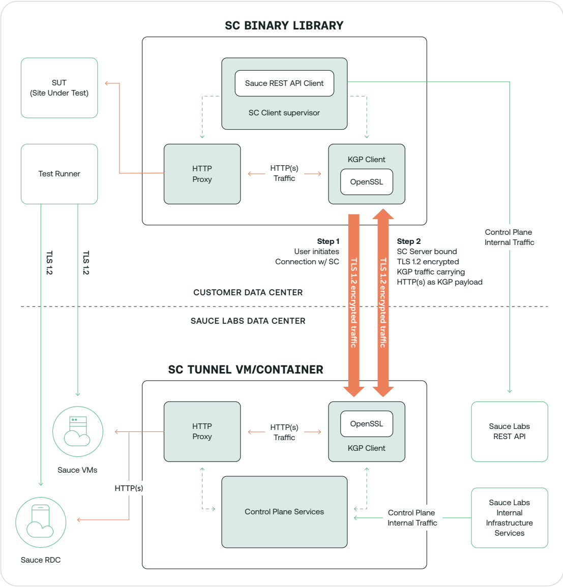
Figure 3: Sauce Connect components interacting with user’s environment
