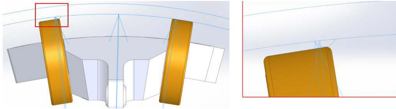
Figure 8 – Schematic of sensor carrier with wheels running on the long seam and generating a tilt of the sensor plate.
