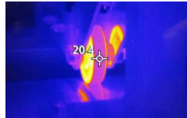
Figure 15 – Thermal image of polyurethane sensor carrier wheel during proof-of-concept testing (°C)
