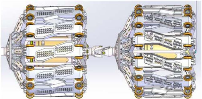
Figure 5 – Initial tool design with electronics modules inside sensor carrier frame and long sensor holders.
