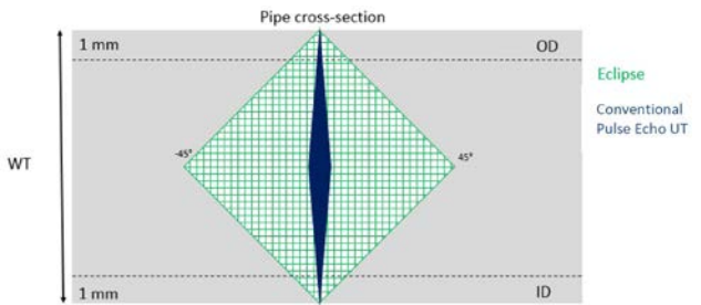
Figure 2 – Conventional Pulse Echo and Eclipse off-radius capabilities
