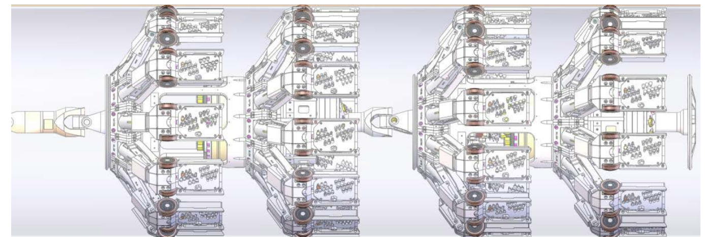
Figure 11 – Schematic of the 36" sensor carrier design inside a pipeline
