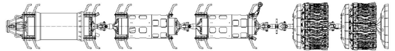
Figure 6 – Conventional tool design with cascaded electronics modules.
