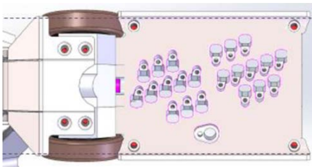
Figure 9 – Schematic of redesigned, shorter sensor plate
