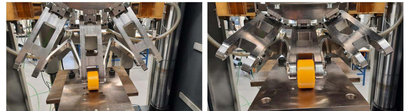
Figure 12 – Synchronous tests of springs
