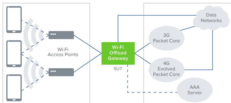
Figure 1. Wi-Fi Offloading with 3GPP.
