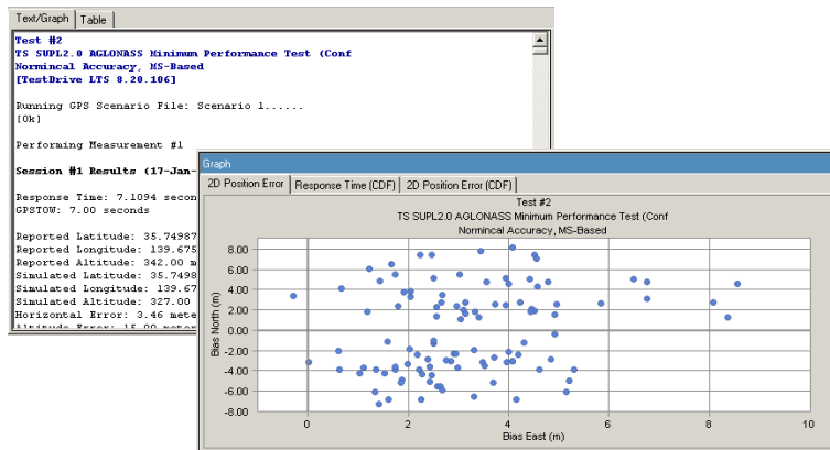
Sample results from SUPL 2.0 A-GLONASS minimum performance testing
