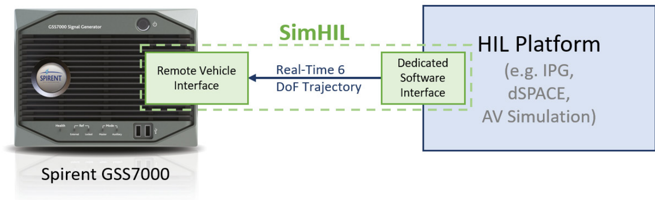
Figure 1: SimHIL Overview
