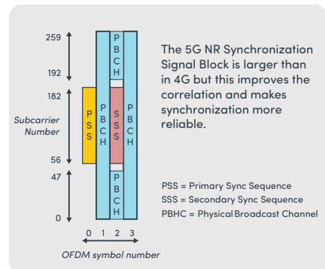
Figure 3. 5G NR SSB structure
