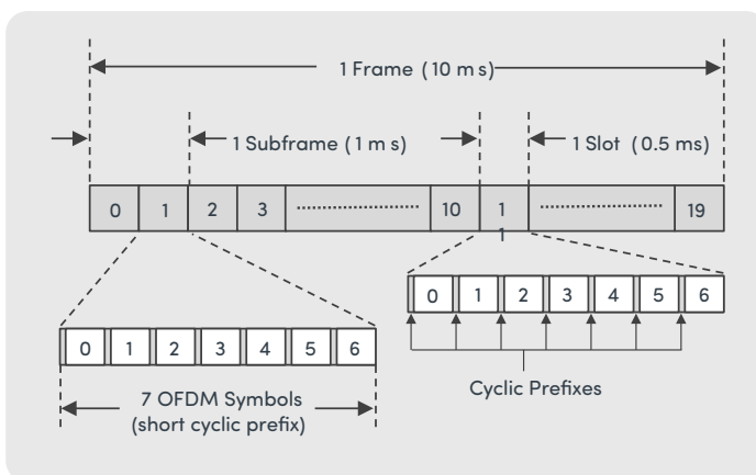
Figure 1. LTE Frame Structure
