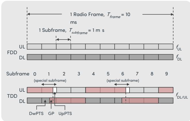
Figure 2. Comparison of FDD and TDD Frame Structures
