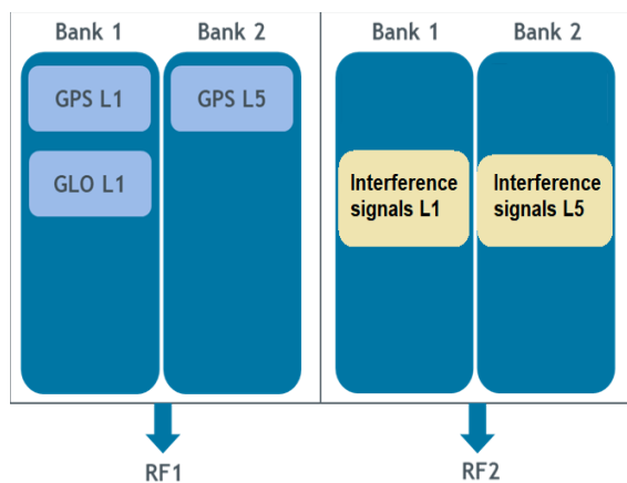
Figure 12 Dual-frequency, GNSS + interference 2RF system
