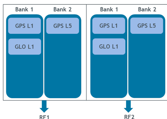
Figure 11 Dual-frequency, 2-constellation 2RF system
