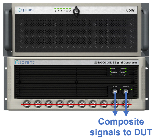
Figure 2 GSS9790 composite mode
