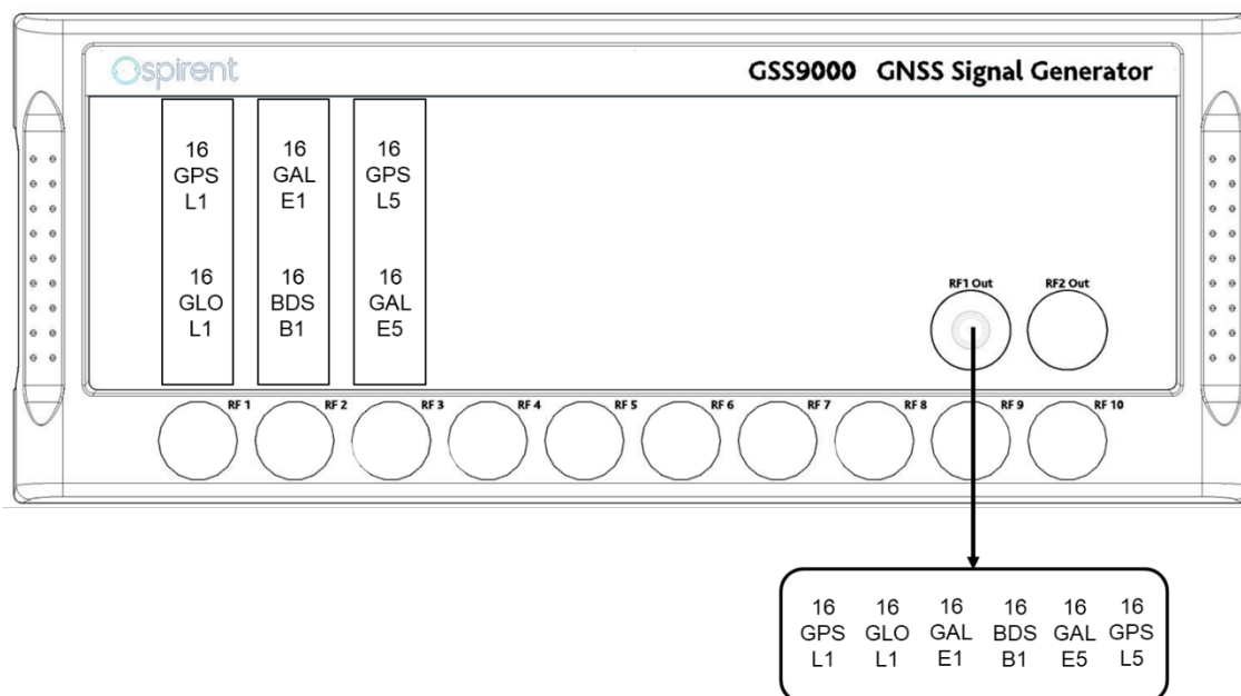
Figure 5 Example of a single output, 3-bank system
