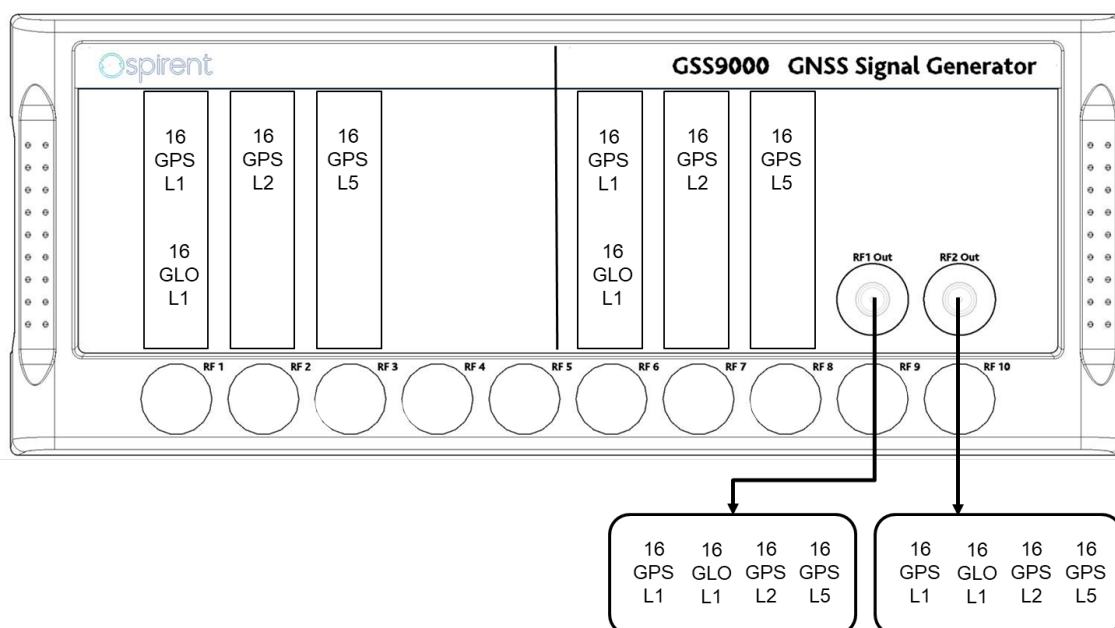
Figure 6 Example of a dual-RF Output, 6-bank system
