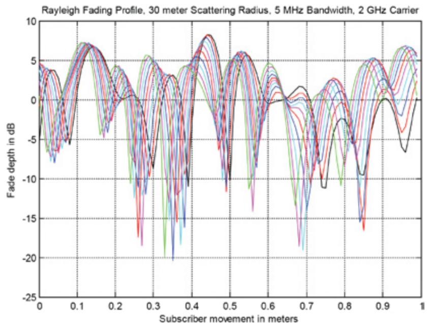
Figure 5: Sample Rayleigh-Faded 5MHz wide signal.
