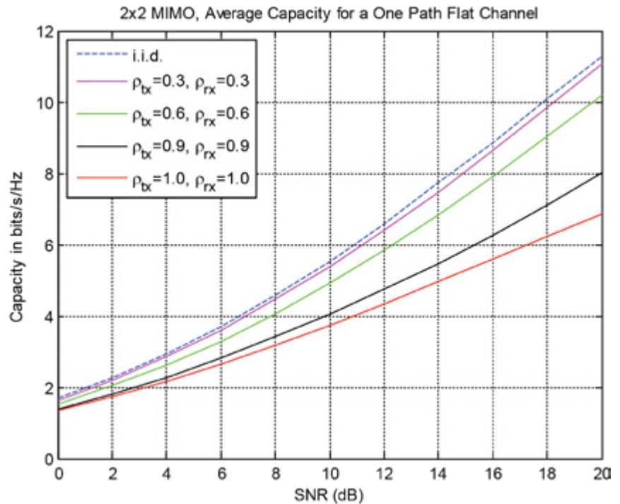
Figure 18: Average MIMO capacity.
