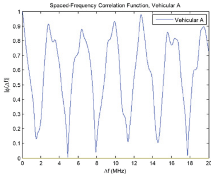
Figure 16: Spaced-frequency correlation function.
