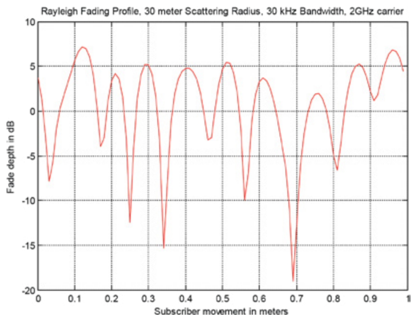
Figure 4: Sample Rayleigh-Faded narrowband 30kHz signal.
