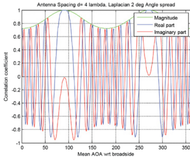
Figure 13: Base station antenna correlation.
