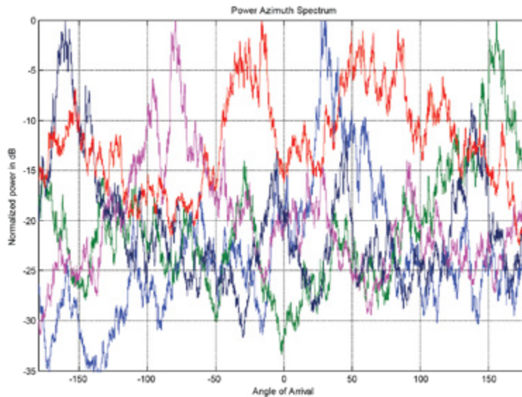
Figure 2: Conceptual Power Azimuth Spectrum for a wide bandwidth signal.
