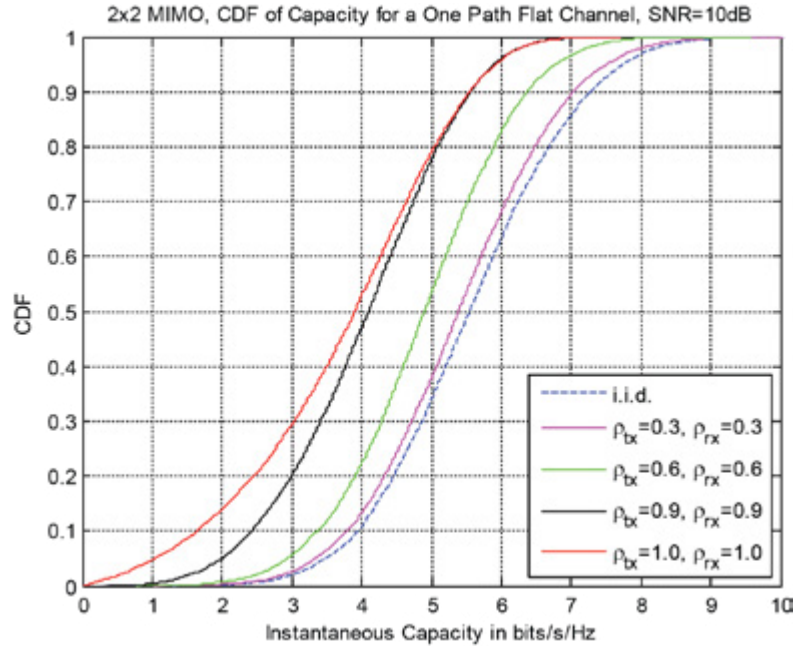
Figure 17: Instantaneous MIMO capacity.
