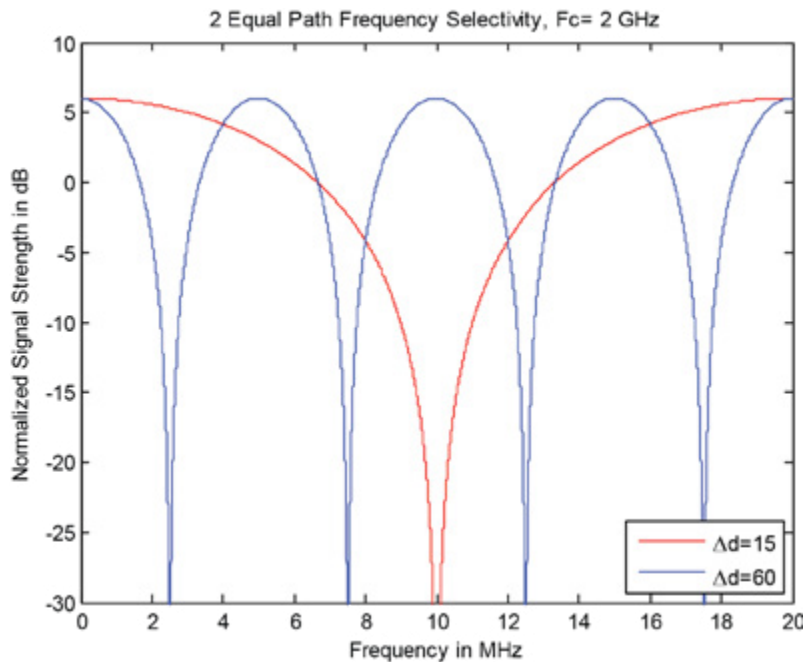
Figure 7: Frequency selective fading for some path length differences.
