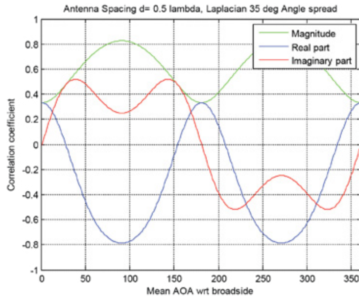
Figure 14: Subscriber antenna correlation.
