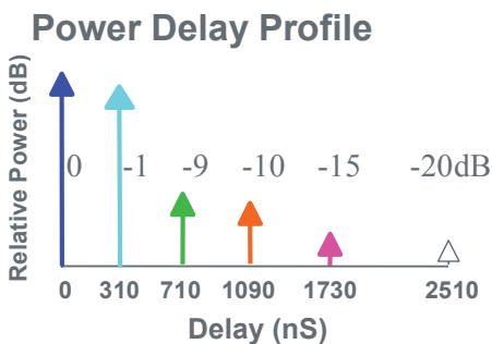
Figure 10: Sample power delay profile from the ITU Vehicular A Channel Model.
