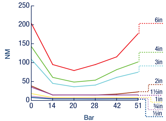
Operation under pressure (differential pressure) – Torque Test
