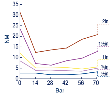
Operation under pressure (differential pressure) – Torque Test
