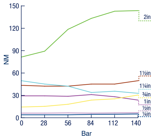
Operation under pressure (differential pressure) – Torque Test
