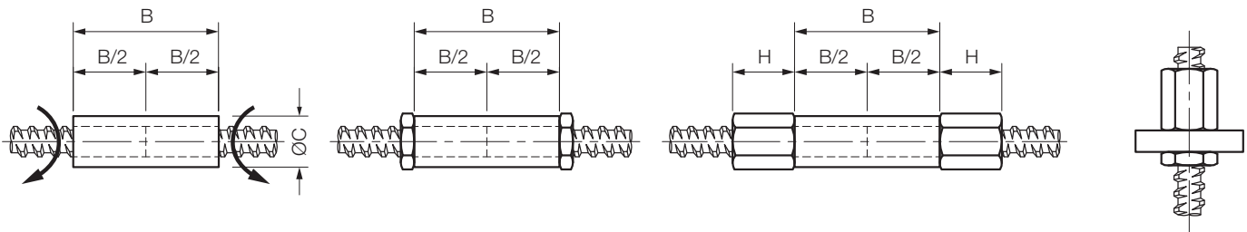
DYWIDAG THREADBAR® – Reinforcing Steel Hardware Dimensions
