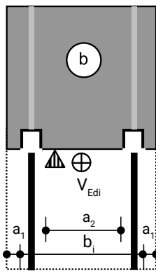
a1 < 50 mm a2 ≥ 50 mm where surface finish is according to DIN EN 1992-1-1, 6.2.5
