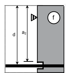
a2 ≥ 50 mm where surface roughness according to DIN EN 1992-1-1, 6.2.5 (see Table 1)
