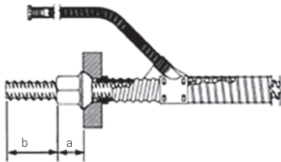
Plate anchorage
