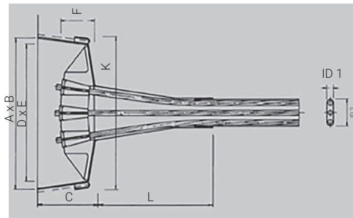
Flat anchorage FA
