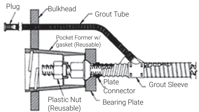
Pocket former detail
