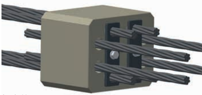
Coupler M
