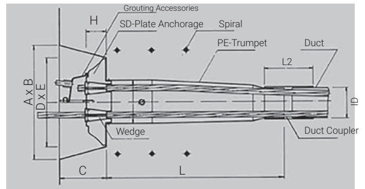
Plate anchorage SD
