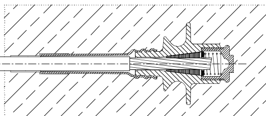
Fixed anchor SF6
