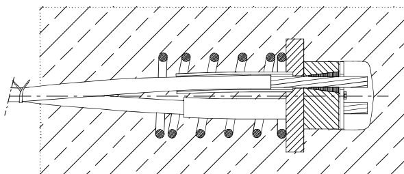
Fixed anchor MEF6
