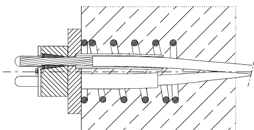
Stressing anchor MER6
