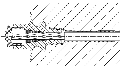
Stressing anchor SK6
