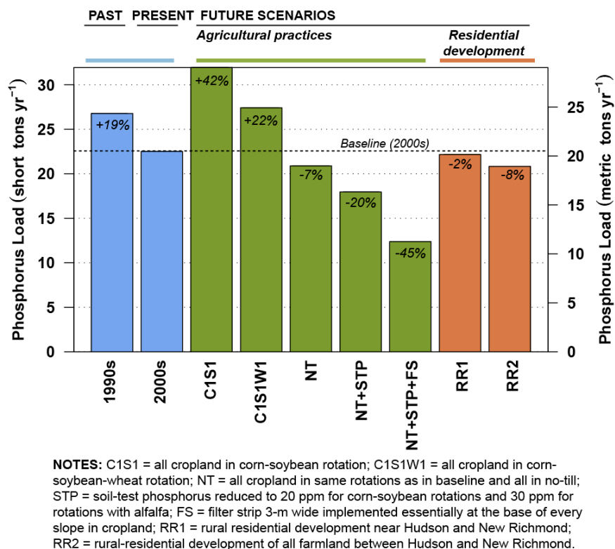
Figure 5. Export of phosphorus from the Willow River watershed under selected scenarios.
